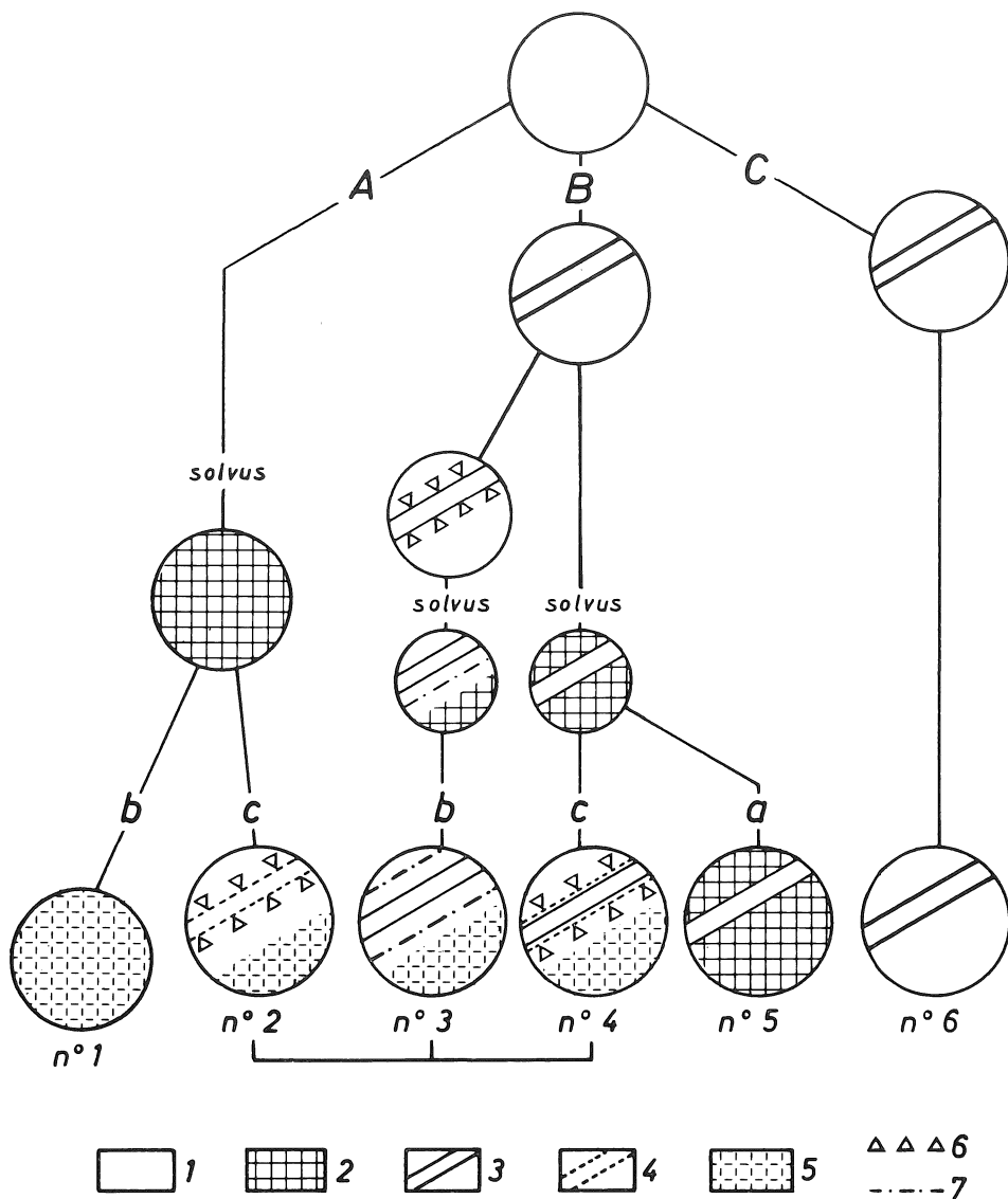
Fig. 3. — Schematic synthesis of the different modes of oxidation of a Ti-rich magnetite leading by decreasing temperature to the different types of microtextures observed. Above, magnetite at high temperature (homogeneous ulvöspinel-rich solid solution). Below, the different types of observed microtextures (n° 1 to n° 6).
