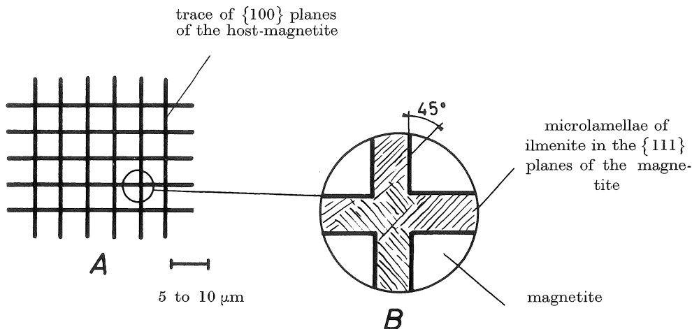
Fig. 2. — Cloth microtexture (section // to {100}).
