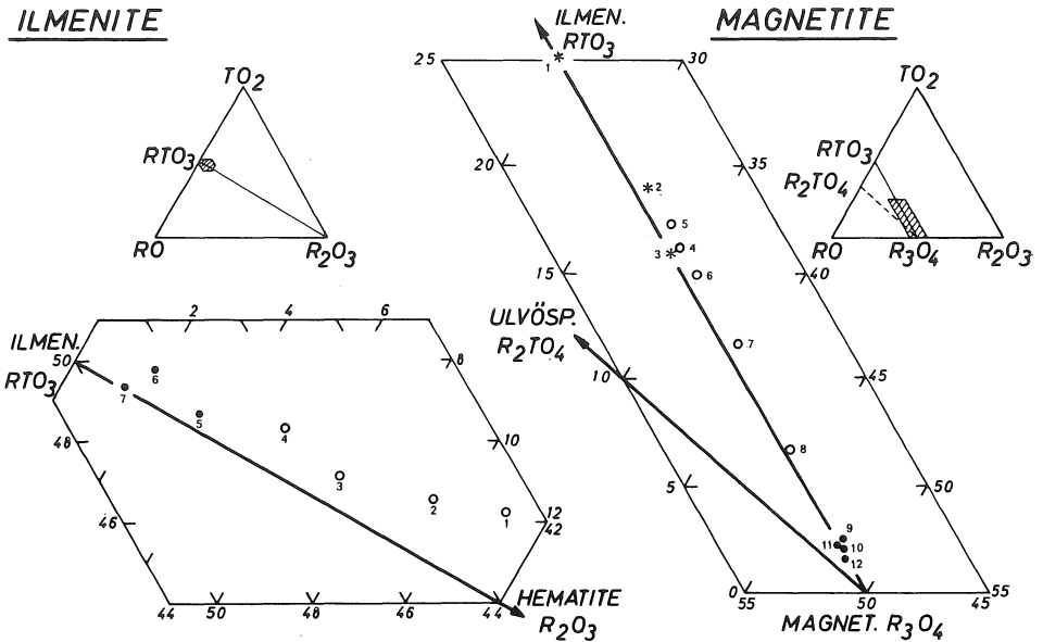
Fig. 1. — Chemical analyses given in Tables 1 and 2 plotted in terms of RO , R_2O_3 , TO_2 (mole percent).
