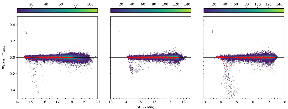
Figure 2: Same as Fig. 1, but confirmed variable sources and sources with unreliable photometry have been removed.
