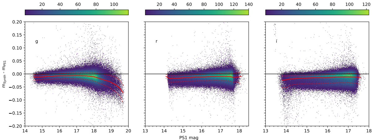
Figure 3: Deviation between Gaia DR3 synthetic magnitude and PS1 magnitude of the crossmatched counterpart. The meaning of the symbols and colourbar is the same as Fig. 1.
