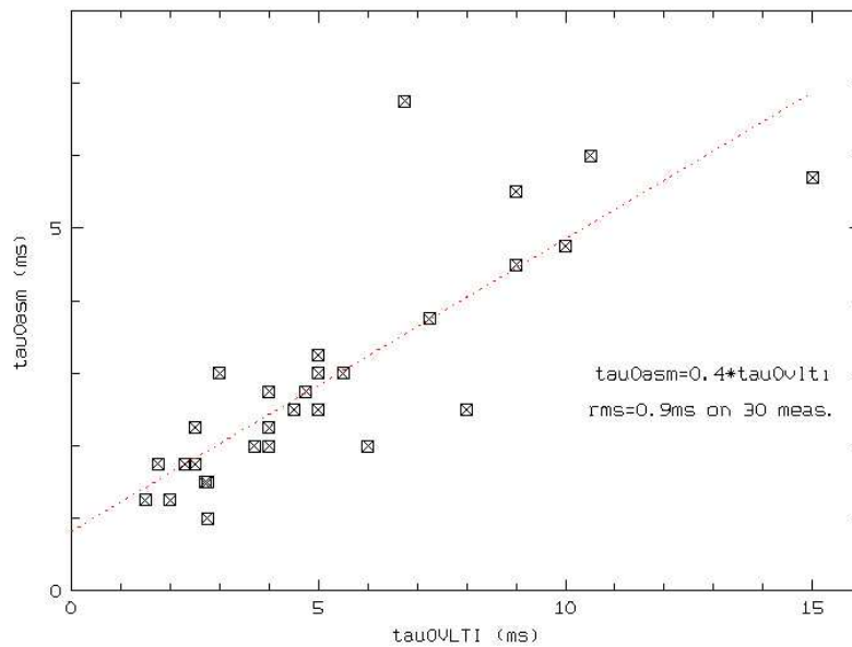
Figure 7: Temporal coherence extracted from VLTI-Vinci power spectra slope analysis (Aug01-Apr02, di Folco et al. (2003)) and as predicted using DIMM seeing and a wavefront velocity V_0 = \text{Max}(V_{ground}, 0.4V_{200mb}) . The line corresponds to the ratio of the coefficients in the definitions (see text).
