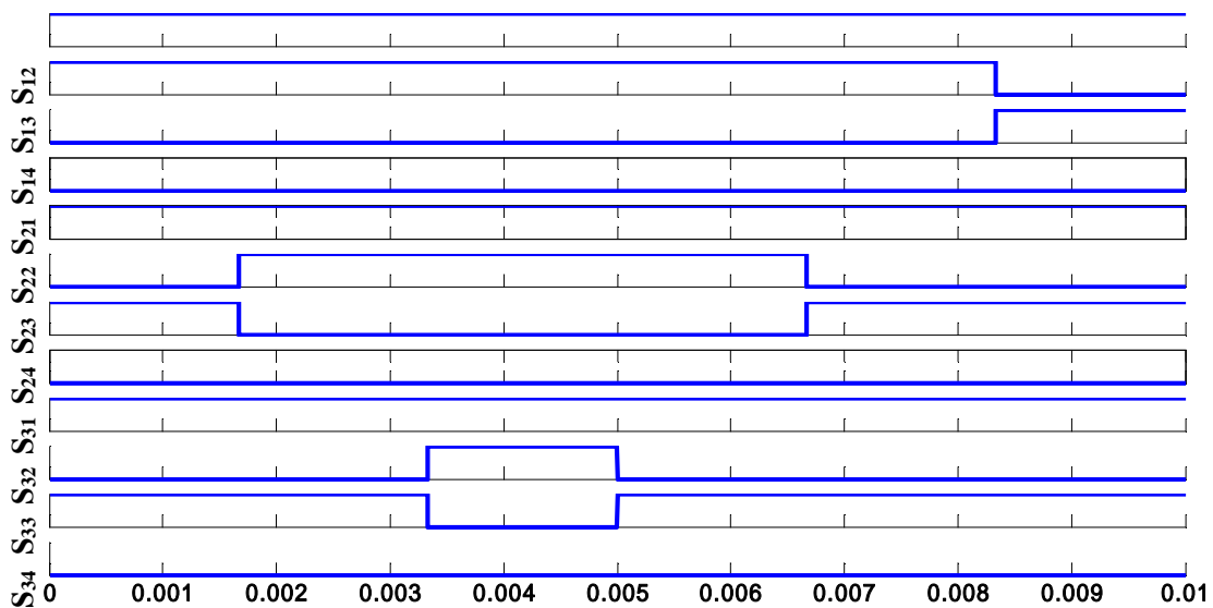
Fig. 4: Gate pulses of switches in implementation of prevalent method for a symmetrical seven level CHB
