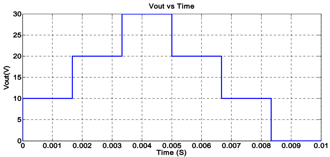
Fig. 3: Output resultant voltage with both prevalent and proposed methods in a symmetrical seven level CHB
