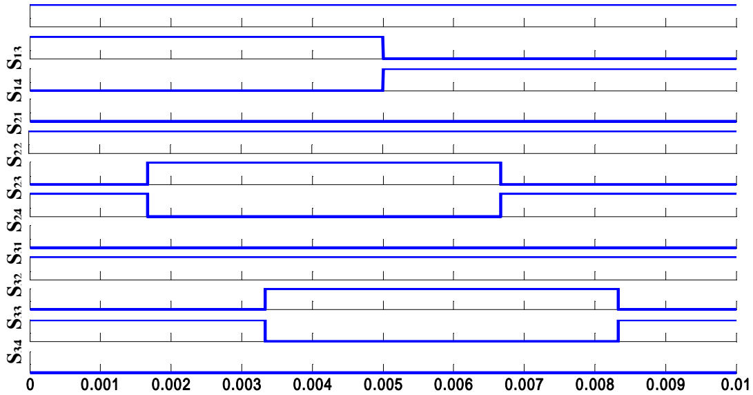
Fig. 5: Gate pulses of switches in implementation of proposed method for a symmetrical seven level CHB
