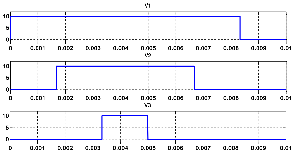
Fig. 6: Usage time of switches for implementation of prevalent method for a symmetrical seven level CHB
