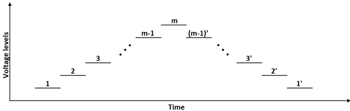
Fig. 1: Generated Voltage levels by a n level converter in positive half cycle
