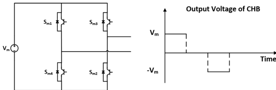
Fig. 2: Number m unit, method of numbering of related switches and output voltage waveform
