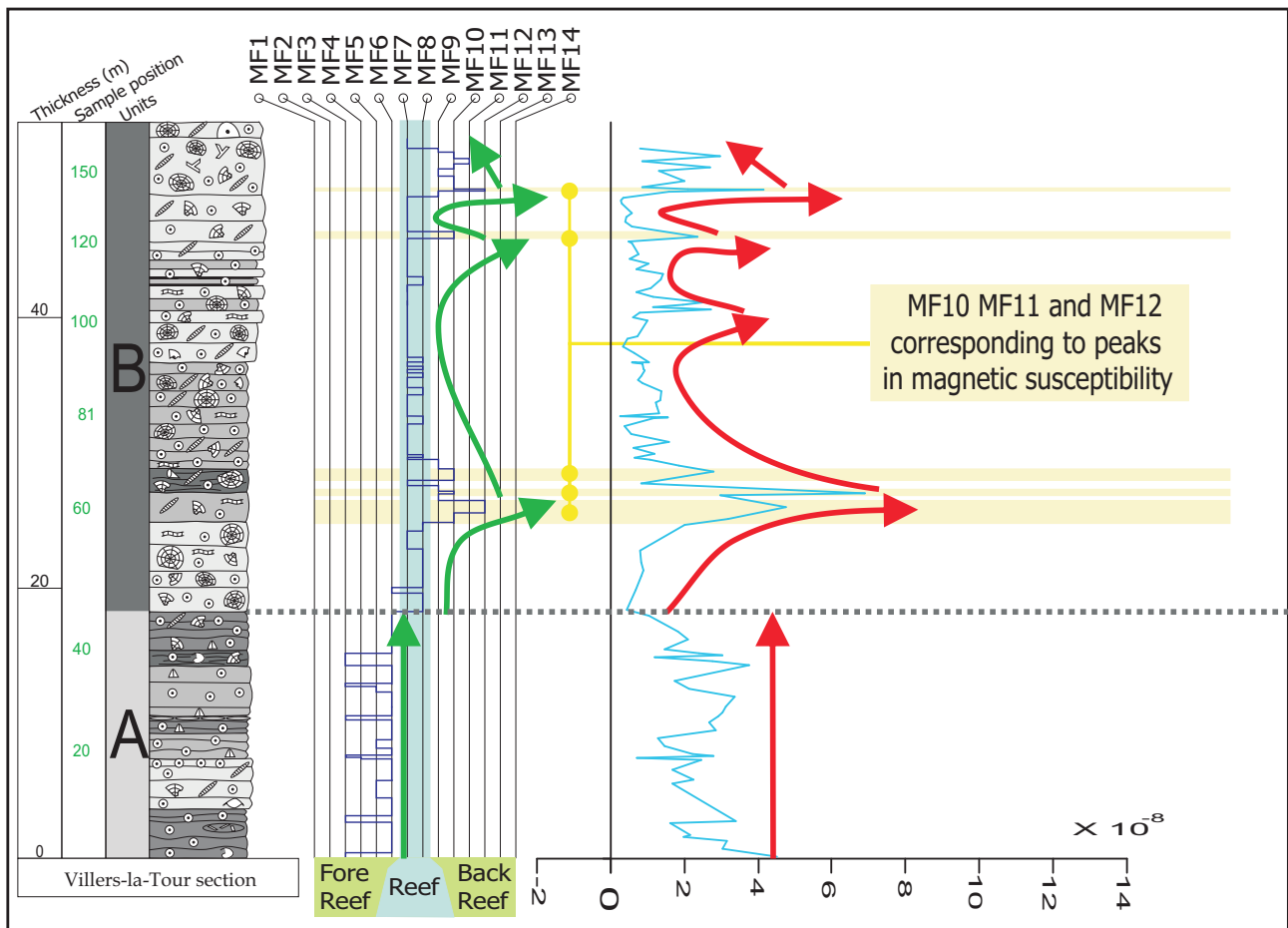
Figure 6: Schematic sedimentological log (see Fig. 5 for legend), lithological units, microfacies curves, and magnetic susceptibility curves of the Villers-la-Tour section. Arrows represent trends in curves.
