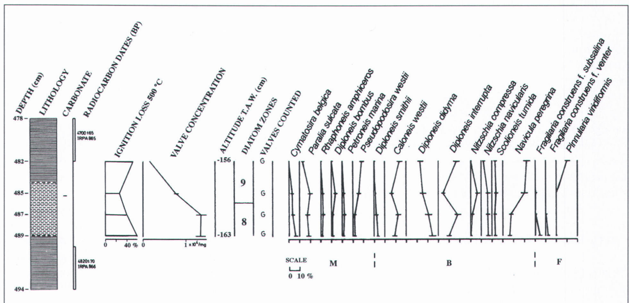
Figure 8. Lithological characteristics, radiocarbon dates, diatom valve concentration and percentage abundance of most important diatom taxa for the lower clayey intercalation in the upper peat of the core Vliegveld (diatom zones 8 and 9; number of valves counted: G - 600-799). M - marine, B - brackish, F - fresh). See Fig. 6 for lithological legend.
