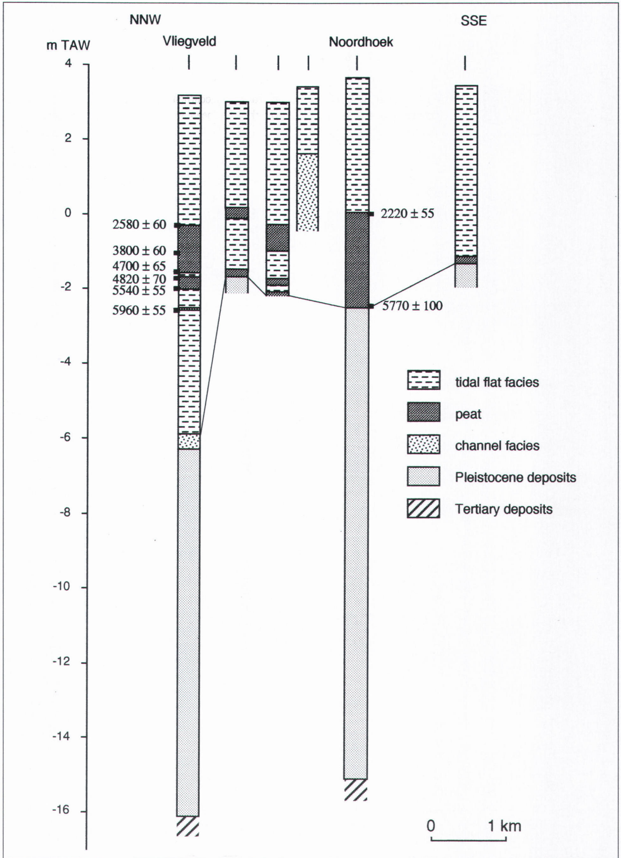
Figure 2. General lithological transect (position indicated on Fig. 1) perpendicular to the coastline with the sites Vliegveld and Noordhoek (radiocarbon dates in yrs BP).
