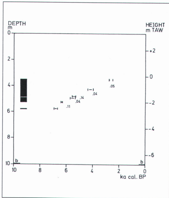
Figure 3. Time/depth plot of the radiocarbon dates for the core Vliegveld (horizontal lines indicate 1s range, vertical lines delimit 2s range) with interpolated mean accumulation rates (cm/cal. year). Black squares at the left show peat occurrence; b indicates base of Holocene deposits.
