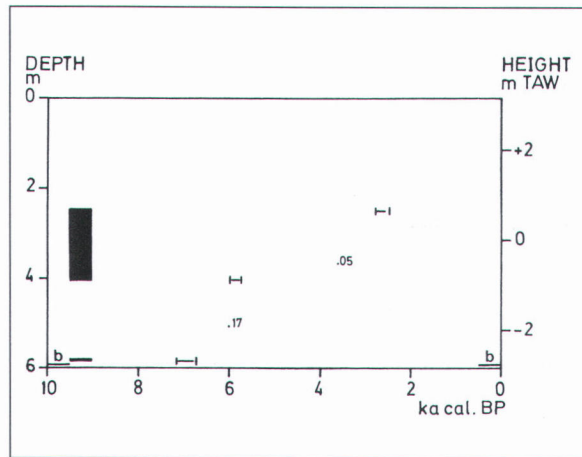
Figure 5. Time/depth plot of the radiocarbon dates for the core Westende 1 (horizontal lines indicate 1s range, vertical lines delimit 2s range) with interpolated mean accumulation rates (cm/cal. year). Black squares at the left show peat occurrence; b indicates base of Holocene deposits.
