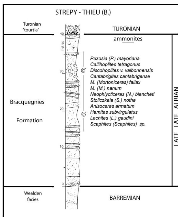
Figure 2. Log of the section, temporarily (1989-1990) exposed in the boat lift construction pit at Strépy-Thieu, with indication of provenance of ammonite taxa recorded herein (modified after Amédro, 2002).
