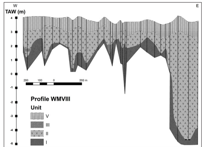
Figure 2. Schematic cross section of the Wijmeers 2 area. Note the well-developed ridge and swale topography of unit I. The base of unit I does not correspond with the lower bounding plane. Unit II is deposited in the channel as well as on the floodplain.
