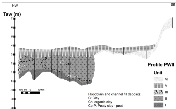
Figure 4. Schematic cross section in the Paardeweide area, with dune deposits bordering the floodplain of the Scheldt River. Note the enlarged lateral extension of the present day floodplain.
