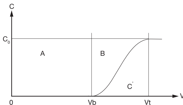
Figure 1. Theoretical breakthrough curve — Courbe de percée théorique.
