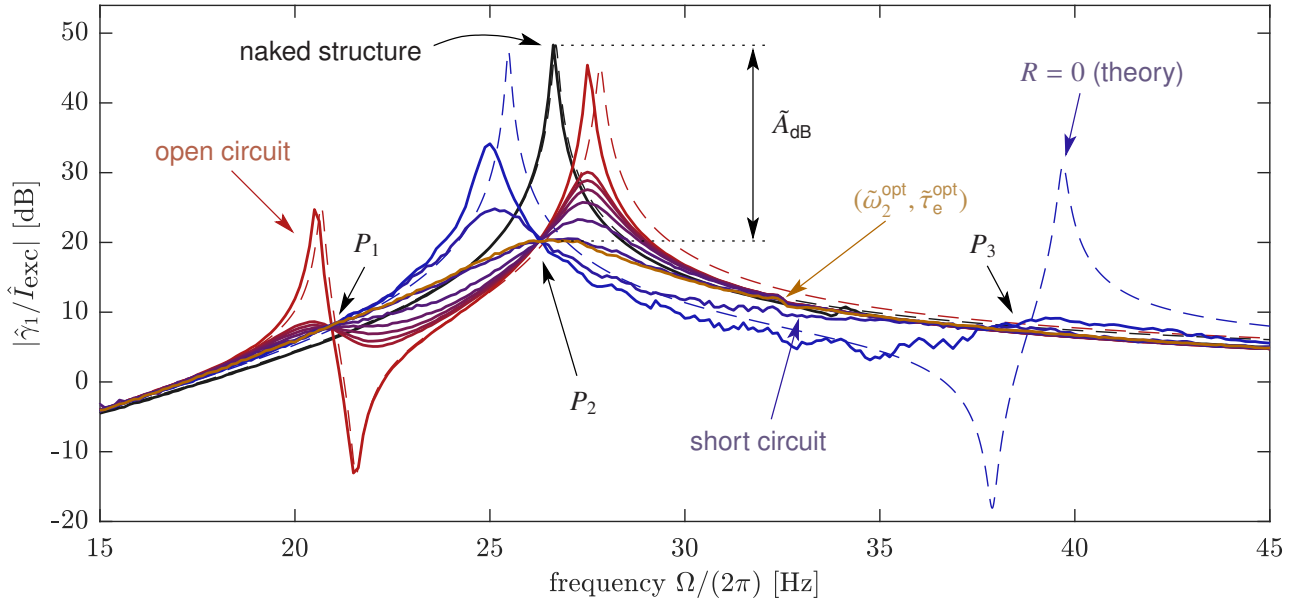
Fig. 23: Experimental modulus of FRF \hat{\gamma}_1/\hat{I}_{exc} of the mechanical structure under several conditions, with the natural frequency of the DVA optimised ( \omega_2 = \tilde{\omega}_2^{opt} ) and with the real time controller that simulates a negative resistance (Fig. 22). (black line): uncoupled primary structure (without DVA and EM-shunt) and (black dashed line) associated theoretical curve; (red line): transducer in open circuit; (gradient curves from red to blue): different value of R_s ; (red dashed line): theoretical open circuit case; (blue dashed line): theoretical R = 0 case; (gold curve) optimal electrical time constant ( \tau_e = \tilde{\tau}_e^{opt} ).
