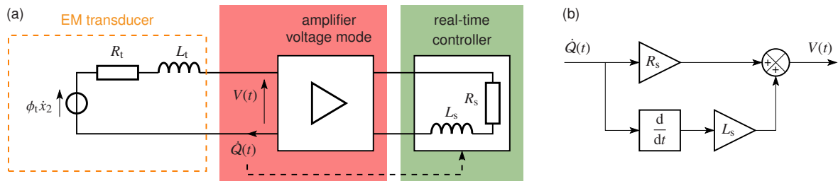
Fig. 24: (a) Diagram of the electrical circuit of the transducer with the simulated resistance and inductance. (b) Block diagram of the real-time controller.
