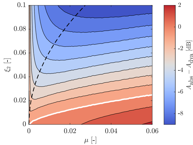
Fig. 18: Evolution of \delta (see Eq. (32)) as a function of \mu and \xi_2 for a primary structure whose damping coefficient is \xi_1 = 0.25\% . The white curve highlights \xi_2(\mu) for which \delta = 0 . The black dashed curve indicates \xi_{dva}(\mu) (Eq. (28)).
