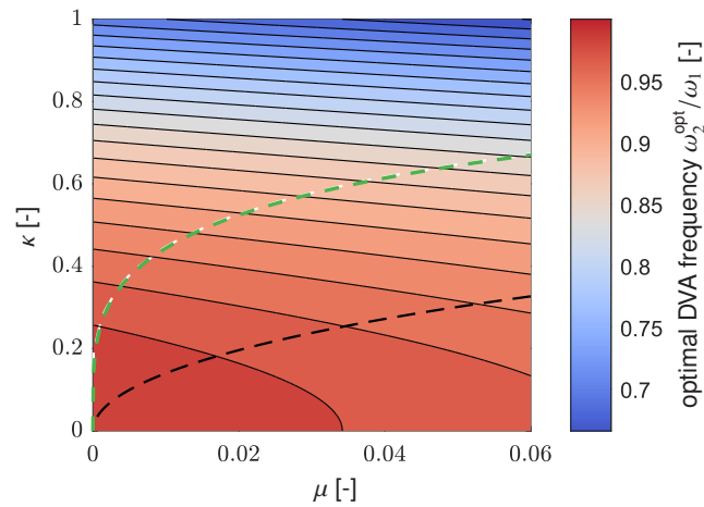
Fig. A.1: Evolution of the ratio \omega_2^{opt}/\omega_1 as a function of \mu and \kappa , shown in Fig. 3. The dashed green curve corresponds to the function of \kappa defined in Eq. (A.6), for which the value of the fixed point P_2 exceeds those of the corrected fixed points P_1 and P_3 .
