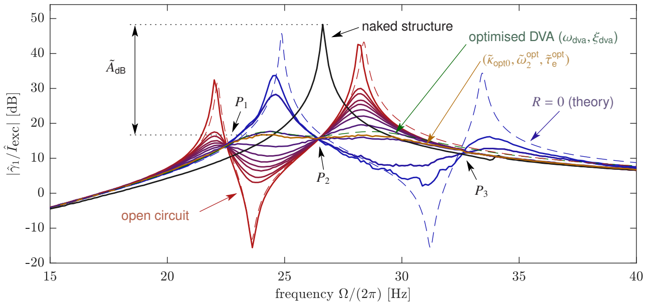
Fig. 25: Experimental modulus of FRF \hat{\gamma}_1/\hat{I}_{\text{exc}} of the mechanical structure under several conditions, with the natural frequency of the DVA and the electromechanical coupling optimised ( \omega_2 = \tilde{\omega}_2^{\text{opt}} , \kappa = \tilde{\kappa}_{\text{opt}} ). (black line): uncoupled primary structure (without DVA and EM-shunt) and (black dashed line) associated theoretical curve; (red line): transducer in open circuit; (gradient curve from red to blue): different values of R_s ; (red dashed line): theoretical open circuit case; (blue dashed line): theoretical R = 0 case; (gold curve) optimal electrical time constant ( \tau_e = \tilde{\tau}_e^{\text{opt}} ); (green dashed line) theoretical optimised mechanical DVA case (its parameters follows Eqs. (37) and (38)).
