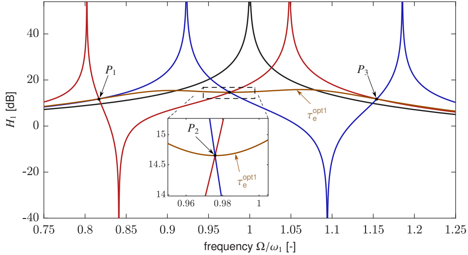
Fig. 5: Modulus of H_1(\Omega) with \xi_1 = \xi_2 = 0 and \omega_2 = \omega_2^{\text{opt}} under several conditions: (black curve): uncoupled primary structure; (red curve): transducer in open circuit ( \tau_e = 0 ); (blue curve): transducer in short circuit ( \tau_e = +\infty ); (gold curve): shunt optimised as \tau_e = \tau_e^{\text{opt1}} . The parameter are \mu = 0.05 and \kappa = 0.7 in order to have the fixed point P_2 above the two others.
