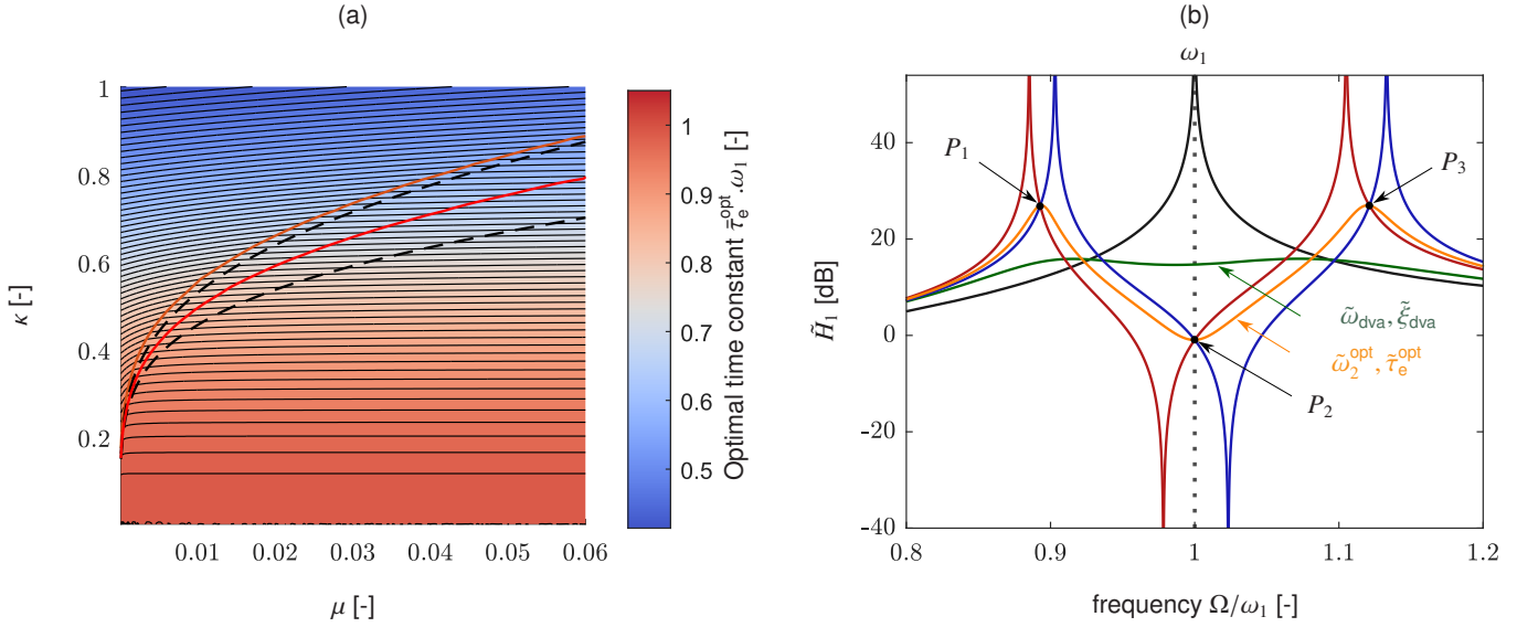
Fig. 20: (a) Evolution of the time constant optimal value \tilde{\tau}_e^{\text{opt}} , scaled by \omega_1 , as a function of (\mu, \kappa) . The red curve shows the optimised value \tilde{\kappa}_{\text{opt}} of \kappa as a function of \mu . The area between the two dashed black curve corresponds to values of (\mu, \kappa) for which the DVA+R-shunt absorber has better performance than a standard mechanical DVA. The orange curve limits the number of extrema of |\tilde{H}_1| : above, it has one maximum and below it has two maxima and one minimum. (b) Modulus of \tilde{H}_1(\Omega) with \xi_1 = \xi_2 = 0 and \omega_2 = \tilde{\omega}_2^{\text{opt}} under several conditions. (black dashed curve): uncoupled primary structure (without DVA and EM-shunt); (red line): transducer in open circuit ( \tau_e = 0 ); (blue line): transducer in short circuit ( \tau_e \rightarrow +\infty ); (orange line): \tau_e = \tilde{\tau}_e^{\text{opt}} = 0.9343/\omega_1 ; (green dashed line) optimised DVA without EM shunt (its parameters follow Eqs. (37) and (38)). The parameters are \mu = 0.05 and \kappa = 0.3 .
