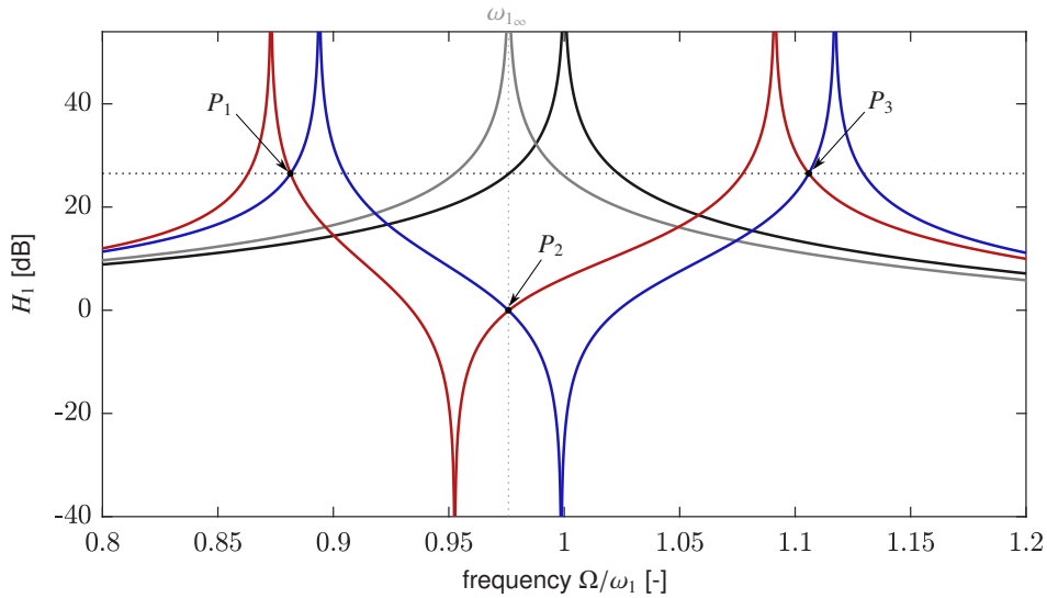
Fig. 4: Modulus of H_1(\Omega) with \xi_1 = \xi_2 = 0 and \omega_2 = \omega_2^{\text{opt}} under several conditions. (black curve): uncoupled primary structure (without DVA and EM-shunt); (grey curve) locked DVA (with k_2 \rightarrow +\infty or c_2 \rightarrow +\infty ); (red curve): transducer in open circuit ( \tau_e = 0 ); (blue curve): transducer in short circuit ( \tau_e = +\infty ). The parameters are \mu = 0.05 and \kappa = 0.3 .
