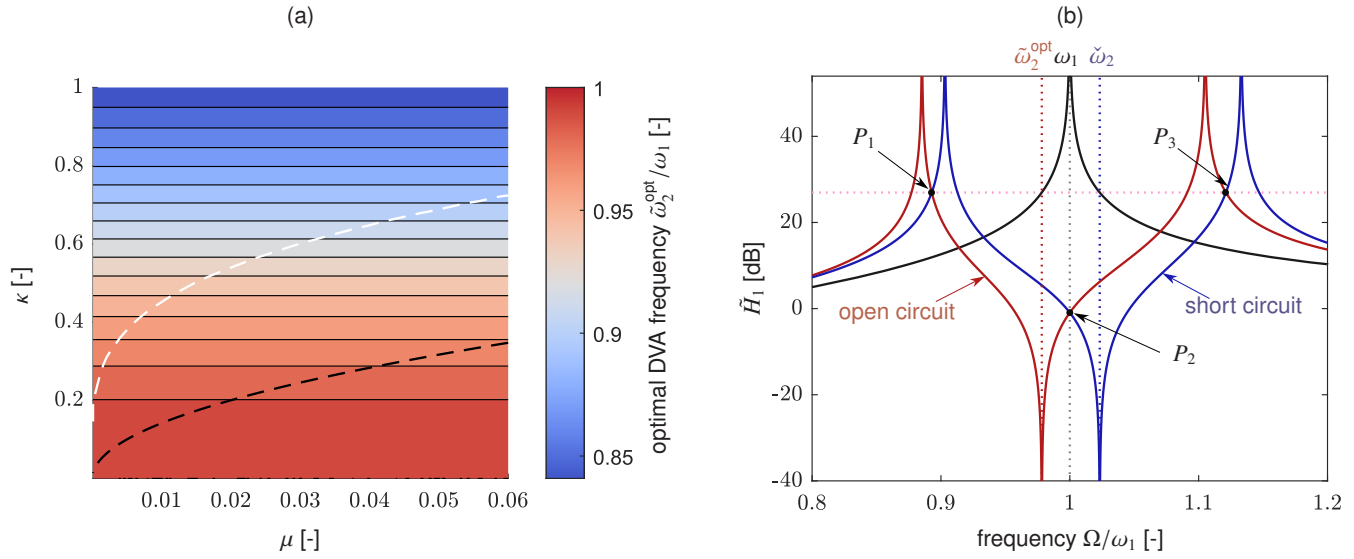
Fig. 19: Optimisation of \omega_2 for the acceleration criterion. (a) Evolution of \tilde{\omega}_2^{\text{opt}}/\omega_1 as a function of \mu and \kappa . The black dashed curve shows the threshold value below which \tilde{\omega}_2^{\text{opt}} exceeds the classical optimal value for a DVA \tilde{\omega}_{\text{dva}} (see Eq. (37)). The white dashed curve marks the threshold above which the amplitude of the central fixed point P_2 is higher than that of P_1 and P_3 . (b) Modulus of \tilde{H}_1 of the system in Fig. 1 with \xi_1 = \xi_2 = 0 and \omega_2 = \tilde{\omega}_2^{\text{opt}} under several conditions. (black dashed curve): uncoupled primary structure (without DVA and EM-shunt); (red curve): transducer in open circuit ( \tau_e = 0 ); (blue curve): transducer in short circuit ( \tau_e = +\infty ). The parameter are \mu = 0.05 and \kappa = 0.3 .
