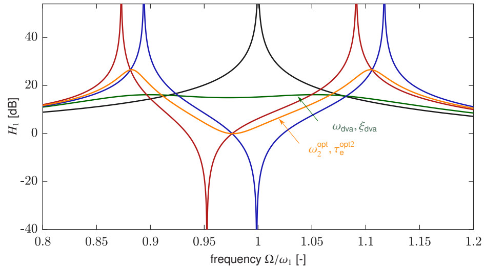
Fig. 10: Modulus of H_1(\Omega) with \xi_1 = \xi_2 = 0 and \omega_2 = \omega_2^{\text{opt}} under several conditions. (black curve): uncoupled primary structure (without DVA and EM-shunt); (red curve): transducer in open circuit ( \tau_e = 0 ); (blue curve): transducer in short circuit ( \tau_e = +\infty ); (orange curve): \tau_e = \tau_e^{\text{opt2}} = 0.9665/\omega_1 . (green dashed curve) optimised DVA without EM shunt (its parameters follow Eqs. (21) and (28)). The parameters are \mu = 0.05 and \kappa = 0.3 .
