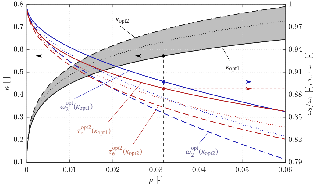
Fig. 16: Tuning graph of a DVA+R-shunt absorber: optimal values \kappa_{\text{opt}} of the EMCF (black curves and left y-axis), that has to be chosen in the gray area, as a function of the mass ratio \mu . Corresponding values of the DVA's natural frequency \omega_2^{\text{opt}} (blue curves) and the electrical time constant \tau_e^{\text{opt2}} (red curves), both scaled by \omega_1 and readable in the right y-axis. The value \kappa_{\text{opt0}} that leads to the best DVA+R-shunt performance is also indicated by the dotted curves.
