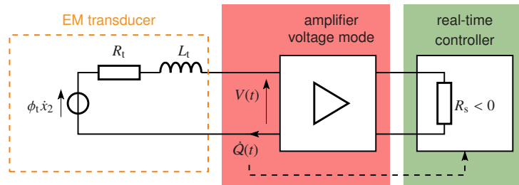
Fig. 22: Diagram of the electrical circuit of the transducer with the simulated resistance.
