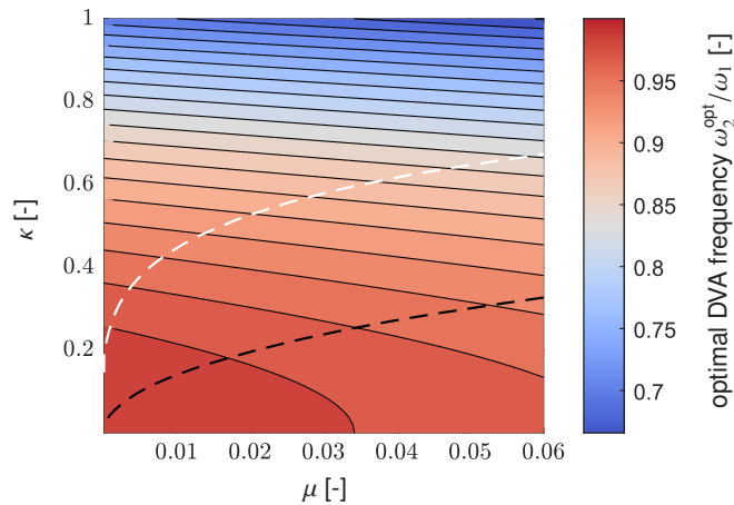
Fig. 3: Evolution of \omega_2^{\text{opt}}/\omega_1 as a function of \mu and \kappa . The black dashed curve shows the threshold value below which \omega_2^{\text{opt}} exceeds the classical optimal value for a DVA \omega_{\text{dva}} (Eq. (21)). The white dashed curve marks the threshold above which the amplitude of the central fixed point P_2 is higher than that of P_1 and P_3 .
