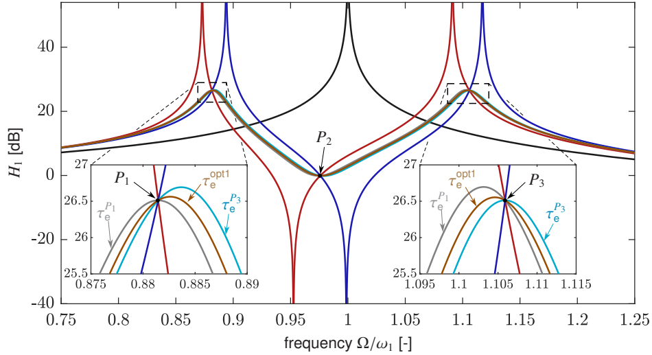
Fig. 6: Modulus of H_1(\Omega) with \xi_1 = \xi_2 = 0 and \omega_2 = \omega_2^{\text{opt}} under several conditions: (black curve): uncoupled primary structure; (red curve): transducer in open circuit ( \tau_e = 0 ); (blue curve): transducer in short circuit ( \tau_e = +\infty ); (grey curve): shunt optimised as \tau_e = \tau_e^{P_1} ; (light blue curve): shunt optimised as \tau_e = \tau_e^{P_3} ; (gold curve): shunt optimised as \tau_e = \tau_e^{\text{opt1}} . The parameter of the DVA are \mu = 0.05 and \kappa = 0.3 , to have the fixed point P_2 below the two others.
