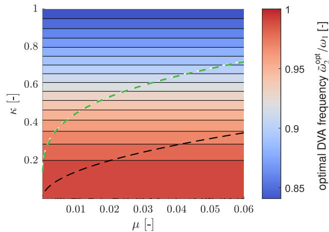
Fig. B.1: Evolution of the ratio \omega_2^{opt}/\omega_1 as a function of \mu and \kappa , shown in Fig. 19. The dashed green curve corresponds to the function of \kappa defined in Eq. (B.4), for which the value of the fixed point P_2 exceeds those of the corrected fixed points P_1 and P_3 .
