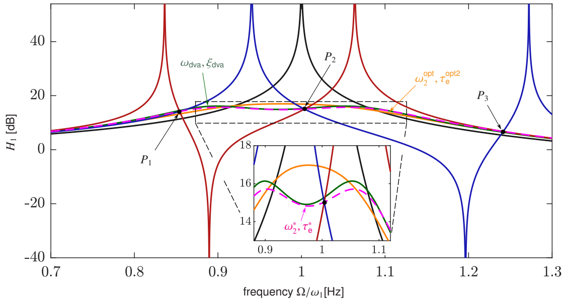
Fig. 13: Modulus of H_1(\Omega) for \xi_1 = \xi_2 = 0 with \mu = 0.05 and \kappa = 0.8 under several conditions. (black curve): uncoupled primary structure (without DVA and EM-shunt); (orange curve): \omega_2 = \omega_2^{\text{opt}} = 0.7951/\omega_1 and \tau_e = \tau_e^{\text{opt2}} = 0.83720/\omega_1 . (green curve) optimised DVA without EM shunt (its parameters follow Eqs. (21) and (28)). The other curves are obtained with \omega_2 = \omega_2^* = 0.8895/\omega_1 under different conditions: (red curve) transducer in open circuit ( \tau_e = 0 ); (blue curve) transducer in short circuit ( \tau_e = +\infty ); (light purple dashed curve) \tau_e = \tau_e^* = 0.4791/\omega_1 .
