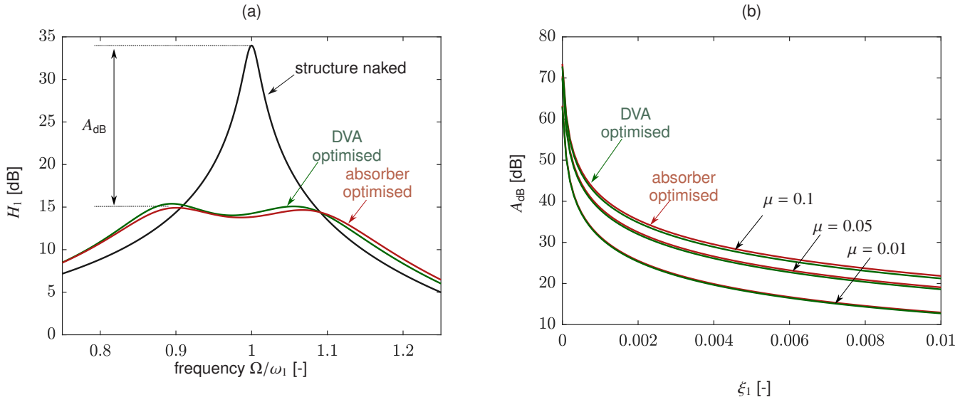
Fig. 17: (a) Modulus of the frequency response function H_1(\Omega) with a non-zero damping coefficient of the primary structure \xi_1 = 1\% , shown under different conditions: (black curve) uncoupled primary structure; (green curve) optimised mechanical DVA ( (\omega_2, \xi_2) = (\omega_{dva}, \xi_{dva}) ); (orange curve) optimised DVA+R-shunt ( (\omega_2, \kappa, \tau_e) = (\omega_2^{opt}, \kappa_{opt}, \tau_e^{opt2}) and \xi_2 = 0 ). (b) Variation of A_{dB} as a function of the damping coefficient \xi_1 of the primary structure and the mass ratio \mu for an optimised mechanical DVA (green curves) and the optimised DVA+R-shunt absorber (orange curves).
