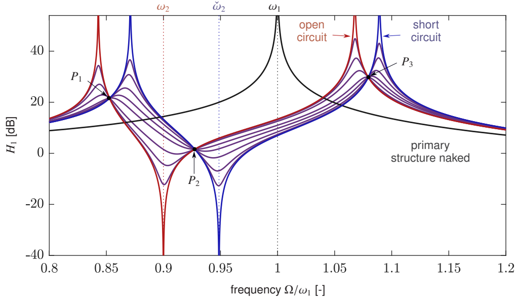
Fig. 2: Modulus of H_1(\Omega) for \xi_1 = \xi_2 = 0 under several conditions. (black curve): uncoupled primary structure (without DVA and EM-shunt); (red curve): transducer in open circuit ( \tau_e = 0 ); (blue curve): transducer in short circuit ( \tau_e = +\infty ); (purple curves): eight values of \tau_e \in [0, +\infty] . The parameters are \omega_2 = 0.9\omega_1 , \mu = 0.05 and \kappa = 0.3 . The dashed vertical curves indicates the extrema of the frequency response while points P_1 , P_2 and P_3 denote the fixed points.
