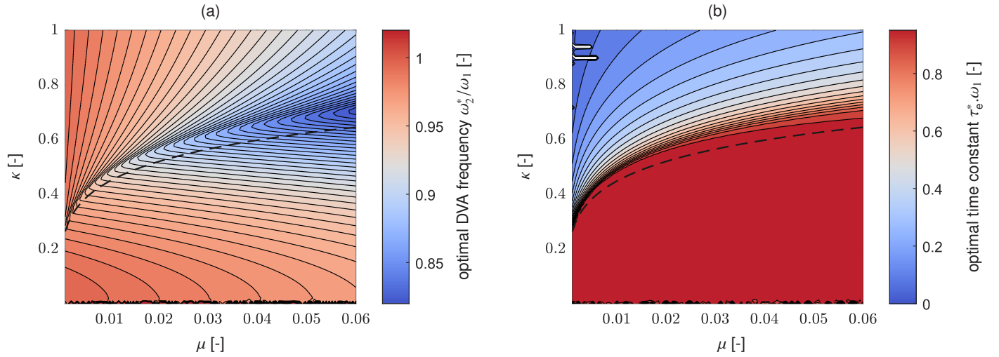
Fig. 15: Evolution of \omega_2^* (a) and \tau_e^* (b), scaled by \omega_1 , as functions of \mu and \kappa . The black dashed line indicates the optimal value \kappa_{opt1} as a function of \mu : above this line, the DVA+R-shunt absorber outperforms a standard mechanical DVA.
