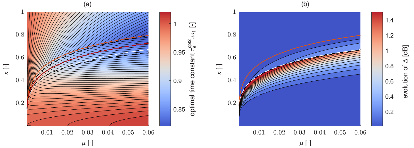
Fig. 8: (a) Evolution of the time constant optimal value \tau_e^{\text{opt}2} , scaled by \omega_1 , as a function (\mu, \kappa) . The red curve shows the optimised value \kappa_{\text{opt}0} of \kappa as a function of \mu . The area between the two dashed black curve corresponds to values of (\mu, \kappa) for which the DVA+R-shunt absorber has better performance than a standard mechanical DVA. (b) Evolution of \Delta (see Eq. (27)) as a function of (\mu, \kappa) . In both plots, the orange curve limits the number of extrema of |H_1(\Omega)| : above, it has one maximum and below it has two maxima and one minimum. The white dashed curve marks the threshold above which the amplitude of the central fixed point P_2 is higher than that of P_1 and P_3 .
