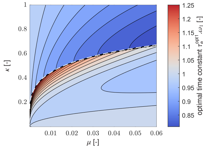
Fig. 7: Evolution of the time constant optimal value \tau_e^{\text{opt1}} , scaled by \omega_1 , as a function of (\mu, \kappa) . The white dashed curve marks the threshold above which the amplitude of the central fixed point P_2 is higher than that of P_1 and P_3 .
