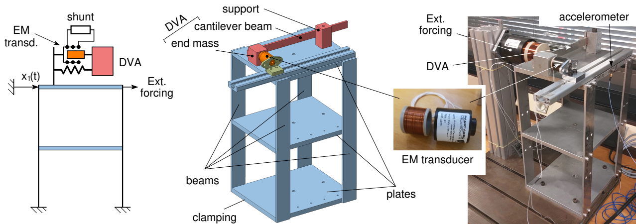
Fig. 21: Diagram and picture of the experimental setup
