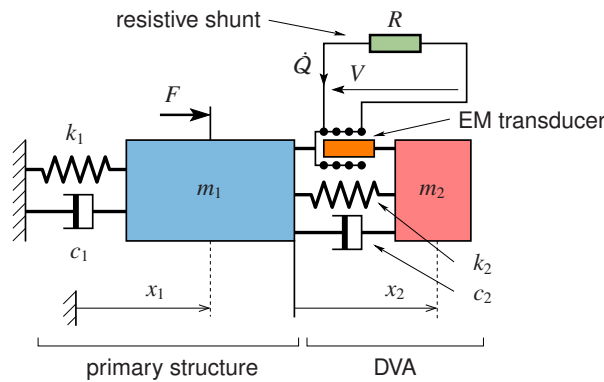
Fig. 1: Diagram of the primary structure coupled to the absorption device composed of a DVA and an electromagnetic resistive shunt between the two mechanical parts.
