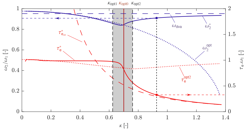
Fig. 14: Evolution of the optimal parameters ( \omega_2 and \tau_e ) as a function of \kappa for \mu = 0.05 . The blue curves show the evolution of \omega_2 , whereas the red curves show the evolution of \tau_e . The solid curves represent (\omega_2^*, \tau_e^*) obtained from numerical optimisation; dotted curves correspond to the parameters obtained using the fixed-point method ( \omega_2^{\text{opt}}, \tau_e^{\text{opt2}} ). The dashed curves indicate the asymptotic values ( \omega_{\text{dva}}, \tau_{e\infty} ).
