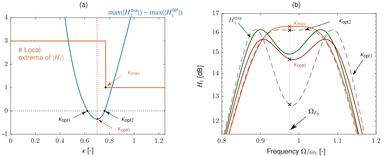
Fig. 12: Remarkable values of \kappa for \mu = 0.05 . (a) The sky-blue curve shows the difference between the maximum modulus of H_1 of the optimised device and that of the optimised DVA. The interval [\kappa_{\text{opt1}}, \kappa_{\text{opt2}}] indicates the range of \kappa where the maximum modulus of H_1 of the device is lower than the maximum FRF of the optimised DVA. The minimum of the sky-blue curve corresponds to \kappa_{\text{opt}} . The orange curve shows the number of stationary points of the FRF of the optimised device. The change in the number of stationary points occurs at \kappa_{\text{max}} . (b) FRFs for different values of \kappa with their corresponding optimised parameters ( \omega_2^{\text{opt}}, \tau_e^{\text{opt}} ). The green curve shows the modulus of H_1 for an optimised DVA.
