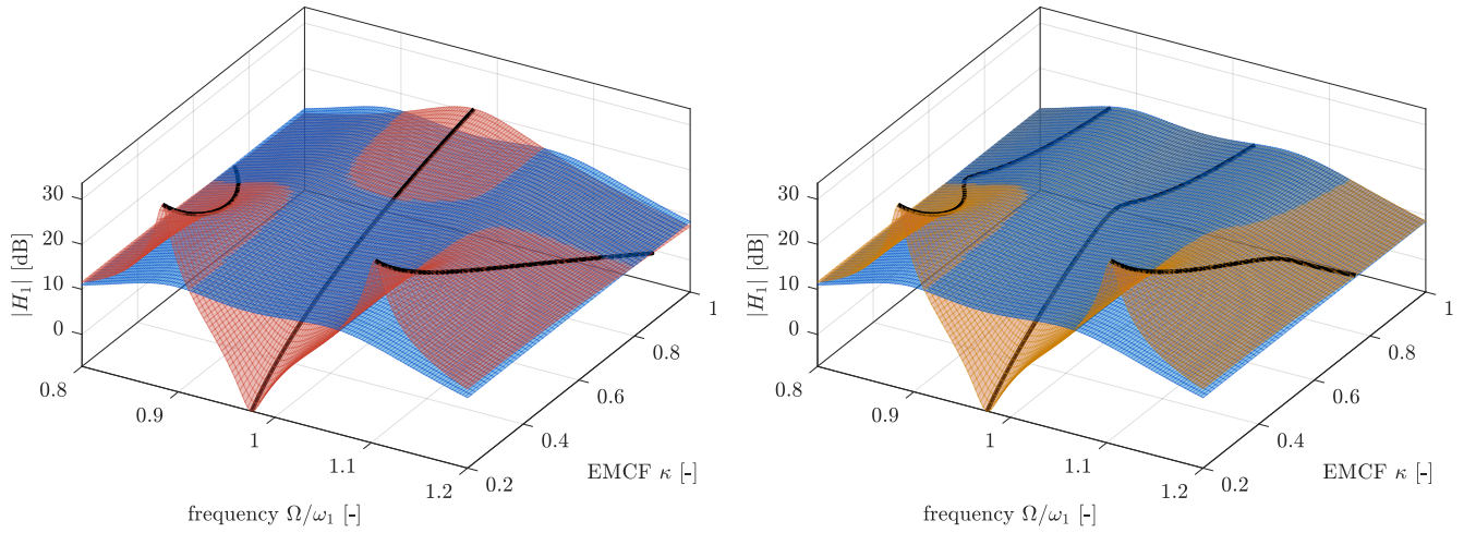
Fig. 11: Variation of the modulus of H_1(\Omega) as a function of the EMCF \kappa . The red surface is the case of a DVA + R-shunt absorber, for \xi_2 = 0 and for optimal values of the parameters \omega_2 = \omega_2^{\text{opt}} and \tau_e = \tau_e^{\text{opt}2} ; the orange surface is the same for optimal values \omega_2 = \omega_2^* and \tau_e = \tau_e^* . The blue surface is the case of an optimal DVA with \omega_2 = \omega_{\text{dva}} and \xi_2 = \xi_{\text{dva}} . In both cases, \xi_1 = 0 and the mass ratio is \mu = 0.05 . The black solid curves are the locus of the fixed points.
