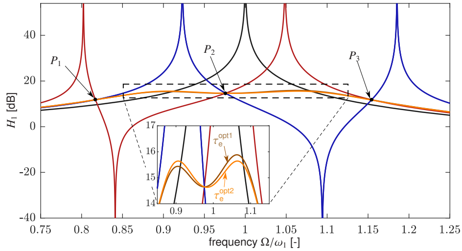
Fig. 9: Modulus of H_1(\Omega) with \xi_1 = \xi_2 = 0 and \omega_2 = \omega_2^{\text{opt}} under several conditions: (black curve): uncoupled primary structure; (red curve): transducer in open circuit ( \tau_e = 0 ); (blue curve): transducer in short circuit ( \tau_e = +\infty ); (gold curve): shunt optimised as \tau_e = \tau_e^{\text{opt1}} ; (orange curve): shunt optimised as \tau_e = \tau_e^{\text{opt2}} . The parameter are \mu = 0.05 and \kappa = 0.7 in order to have the fixed point P_2 above the two others.
