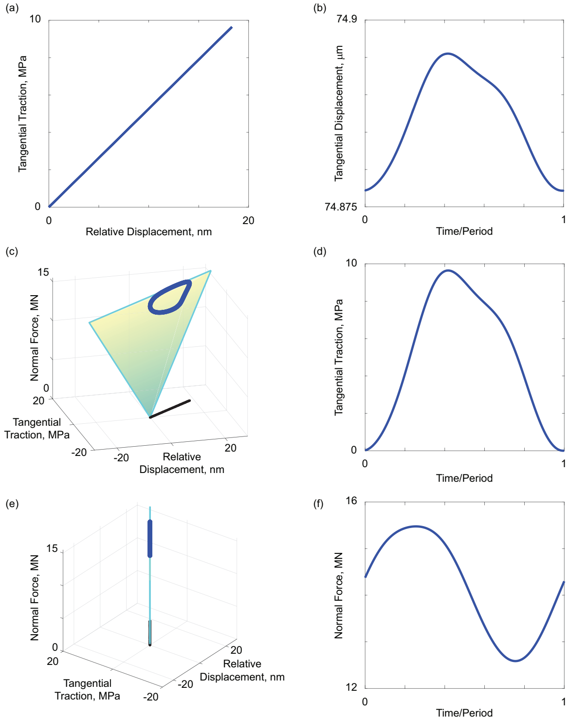
Fig. 14: Hysteretic response of element E (as indicated in Fig. 2) of the Brake-Reuß beam showing the (a) hysteresis loop, (b) original displacement as a function of time normalized by the period of the response, (c) Masing manifold in the displacement-traction-normal force space, (d) traction as a function of normalized time, (e) view of the Masing manifold aligned to show that the response never deviates from it, and (f) normal force as a function of normalized time. For the Masing manifolds, the traction-displacement response is projected on the t_n = 0 plane as a black line. The response itself is indicated as the blue loop.
