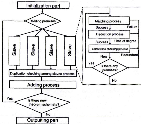
Fig. 1: The model of parallelization version of EnCal
