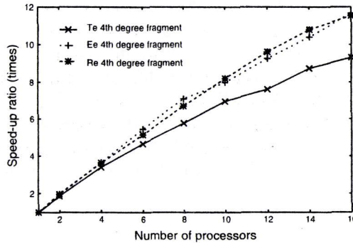
Fig. 3: Speed-up ratio on a clusters of PCs (2 CPU / 1 node)
