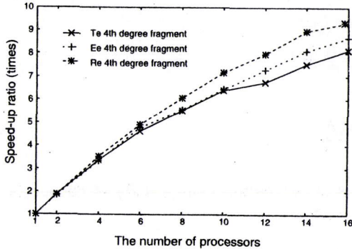
Fig. 2: Speed-up ratio on Sun Enterprise 6000
