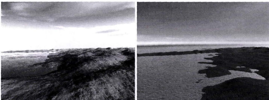
Figure 1. The reconstructions of Titan landscape by M.Zawistowski (Canada) on the basis of the Cassini mission data – see http://www.astrogalaxy.ru/271.html . The seas in the pictures consist of liquid methane mainly . The color of the sky is yellow-orange.
