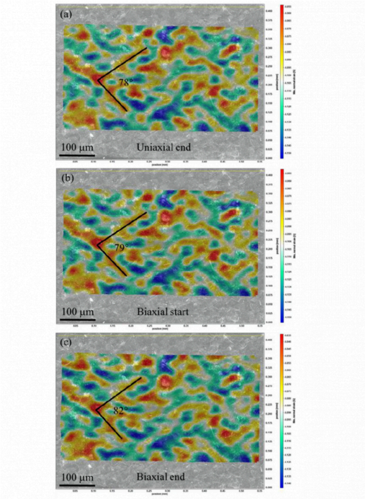
Fig. 8: Y-axis micro strain ( e_y ) distribution at the centre of the specimen calculated from micro DIC analysis after (a) uniaxial end, (b) biaxial start and (c) biaxial end during the continuous strain path change
