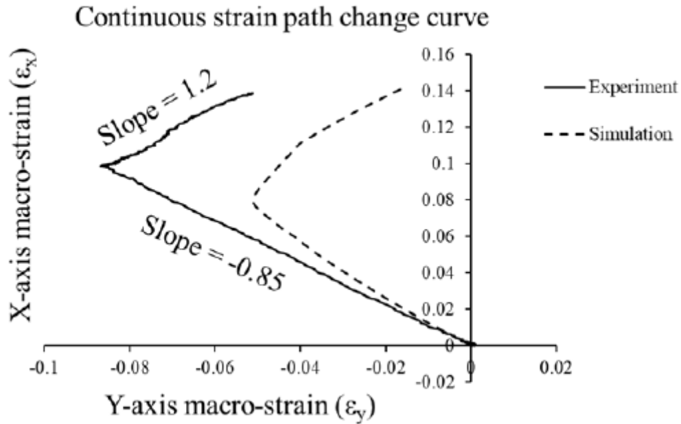
Fig. 6: Experiment vs. simulation continuous strain path change curve of DX54 sample
