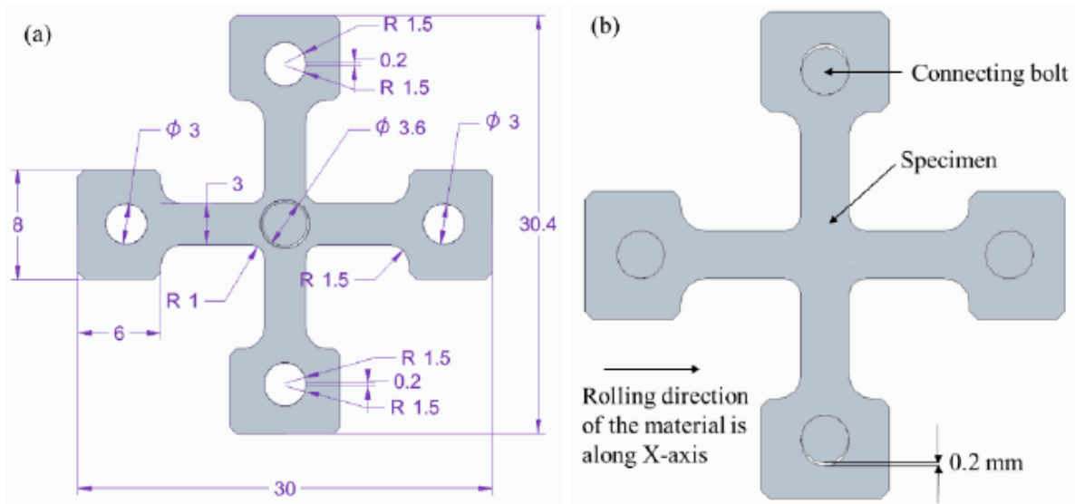
Fig. 2 (a) Design of strain path change specimen and (b) assembly design of connecting bolts and the strain path change specimen showing 0.2 mm travel of connecting bolts in the vertical arms during strain path change
