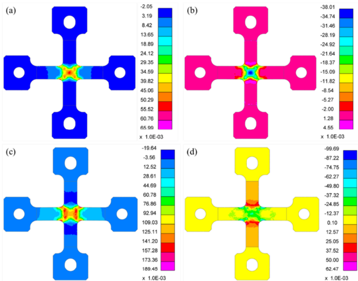
Fig. 4: Simulated macro-strain contour of DX54 specimen during continuous strain path change (a) \epsilon_x and (b) \epsilon_y contour before the strain path change and (c) \epsilon_x and (d) \epsilon_y contour after the strain path change
