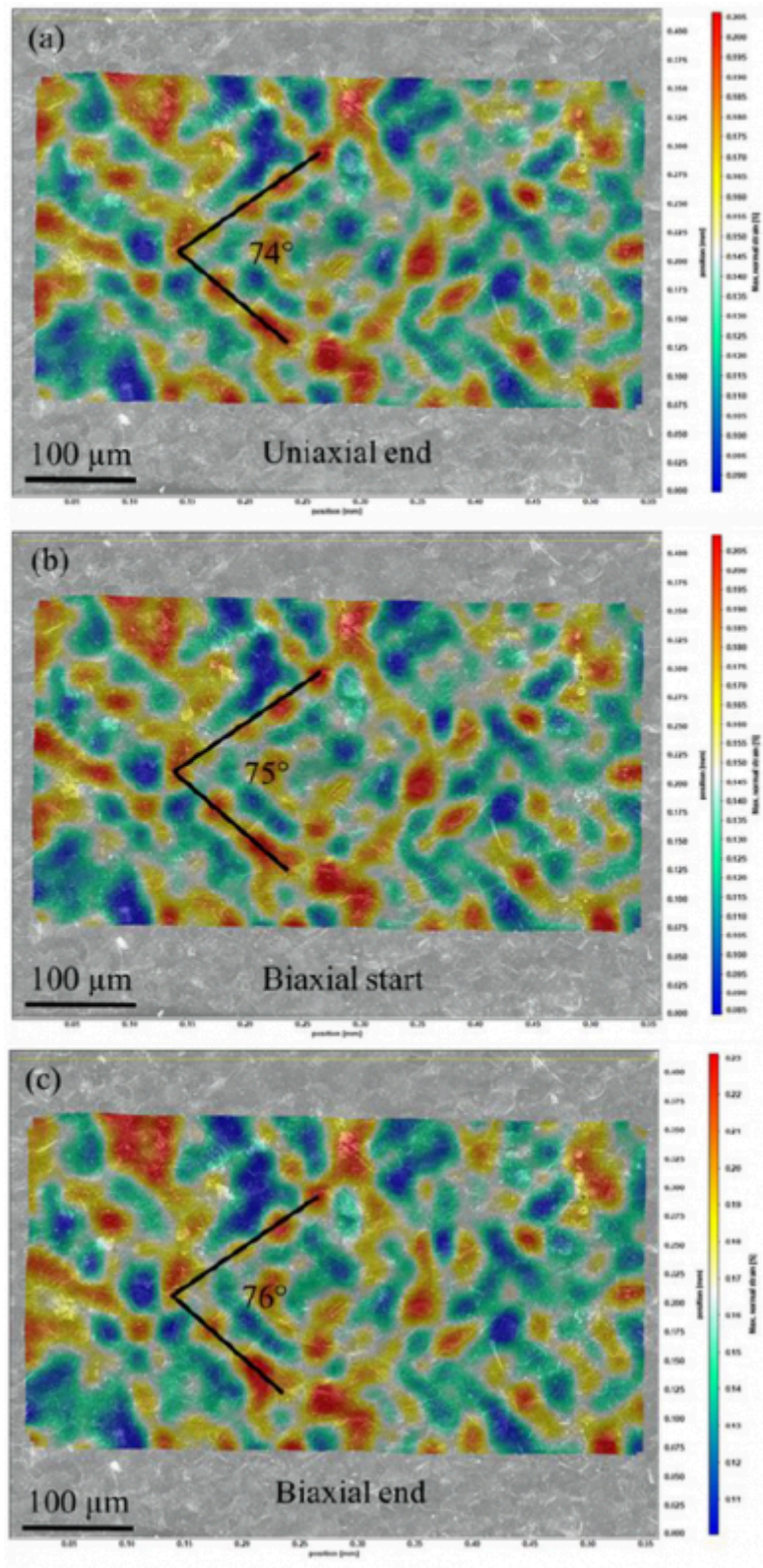
Fig. 7: X-axis micro strain ( \epsilon_x ) distribution at the centre of the specimen calculated from micro DIC analysis after: (a) uniaxial end, (b) biaxial start and (c) biaxial end during the continuous strain path change
