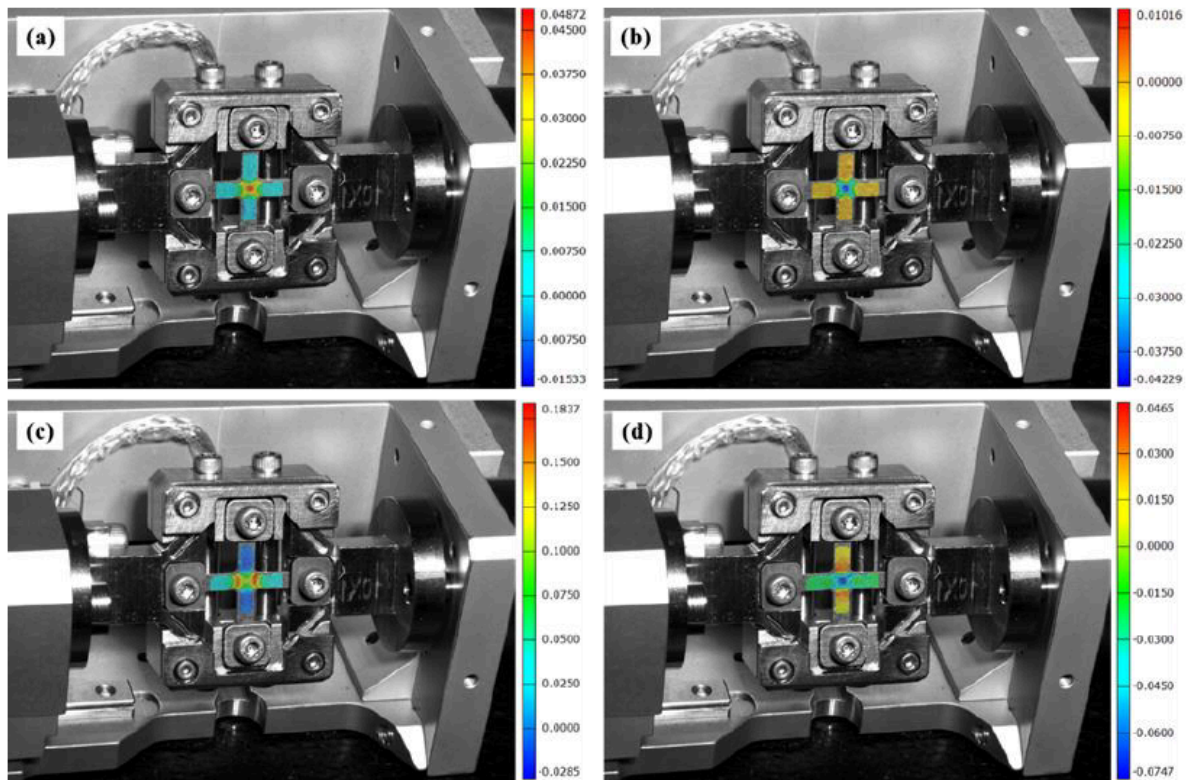
Fig. 5: Experimental macro-strain contour of DX54 specimen during continuous strain path change (a) \epsilon_x and (b) \epsilon_y contour before the strain path change and (c) \epsilon_x and (d) \epsilon_y contour after the strain path change
