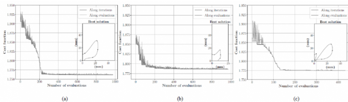
Fig. 3. Cost function evaluation and best obtained solutions' geometry for solution (a) A, (b) B and (c) C
