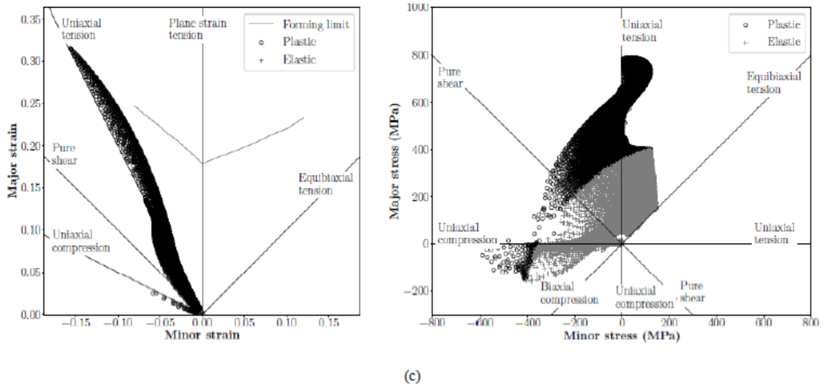
Fig. 4. Minor and major strain and stress diagrams of the best obtained solutions at the moment just before rupture, for solution (a) A, (b) B and (c) C
